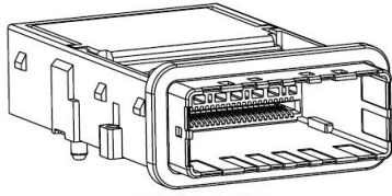
2291931-6/-7 SHOWN UNSPECIFIED DIMENSIONS ARE SAME AS 2291931-1 SCALE 3:1
